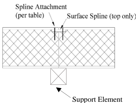
Figure 3a: Interior Support Spline
