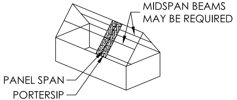
RIDGE BEAM SYSTEM PORTERSIPs SUPPORTED BY THE RIDGE BEAM AND THE EAVE WALLS.
