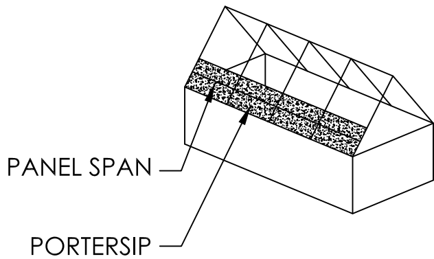
RAFTER SYSTEM PORTERSIPs SUPPORTED BY RAFTERS SPANNING FROM THE RIDGE BEAM TO THE EAVE WALLS.
