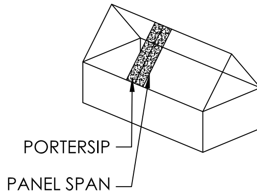
LOAD BEARING WALLS SYSTEM PORTERSIPs SUPPORTED BY RAFTERS SPANNING FROM THE RIDGE BEAM TO THE EAVE WALLS.
