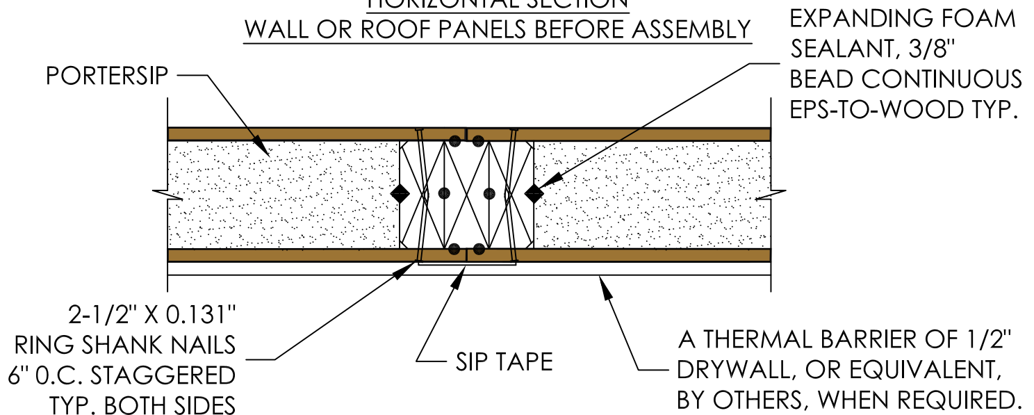
HORIZONTAL SECTION WALL OR ROOF PANELS ASSEMBLED
