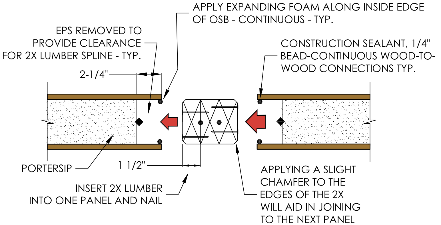
HORIZONTAL SECTION WALL OR ROOF PANELS BEFORE ASSEMBLY
