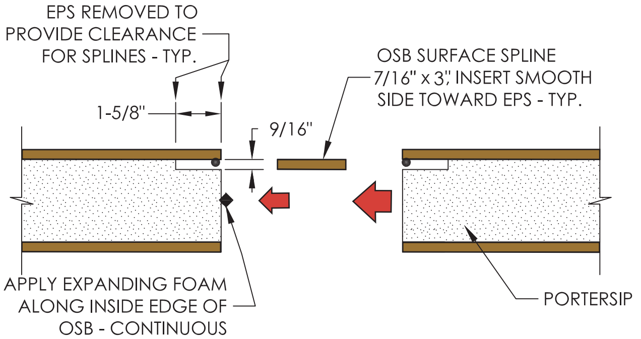
HORIZONTAL SECTION PANELS BEFORE ASSEMBLY
